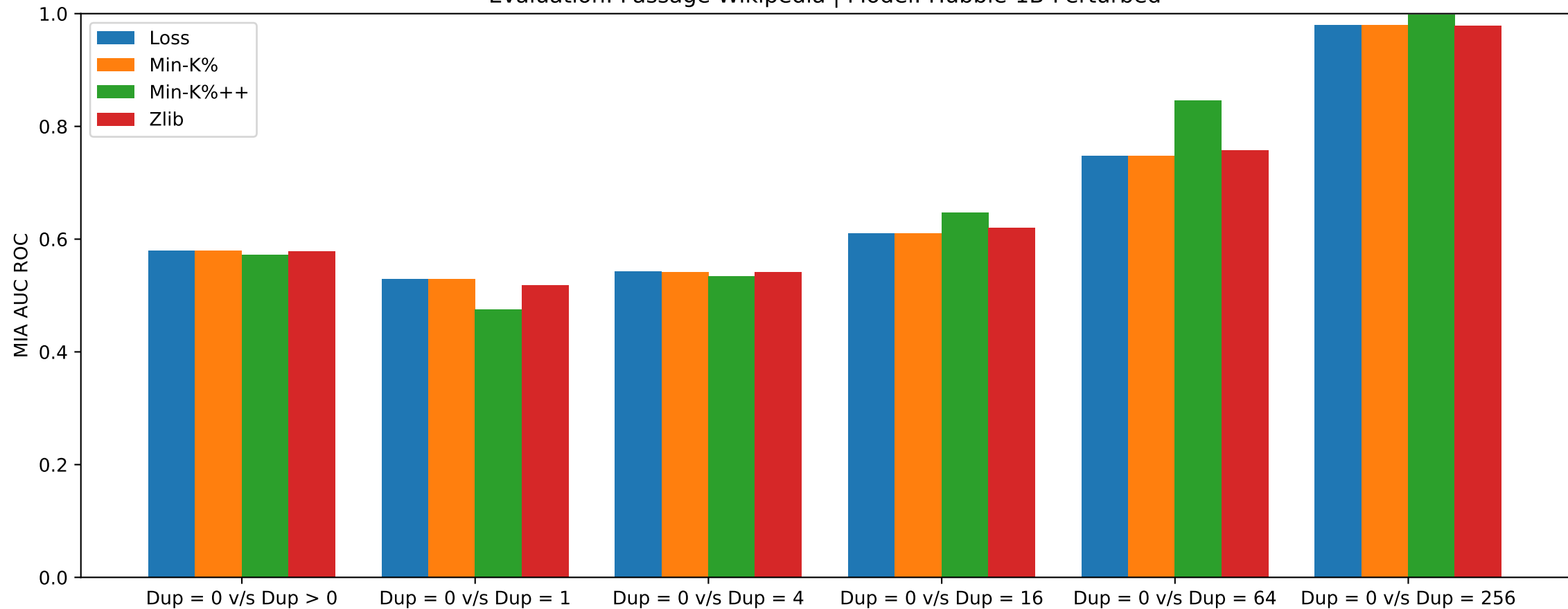
Evaluation: Passage Wikipedia | Model: Hubble-1B-Perturbed
